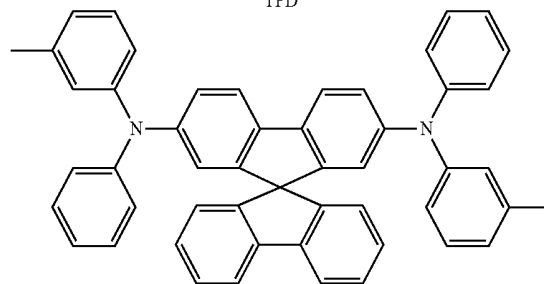
Spiro-TPD
