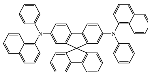
Spiro-NPB
