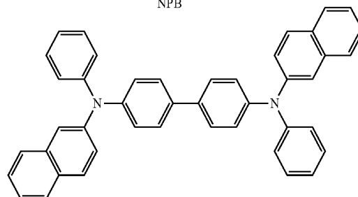
\beta -NPB
